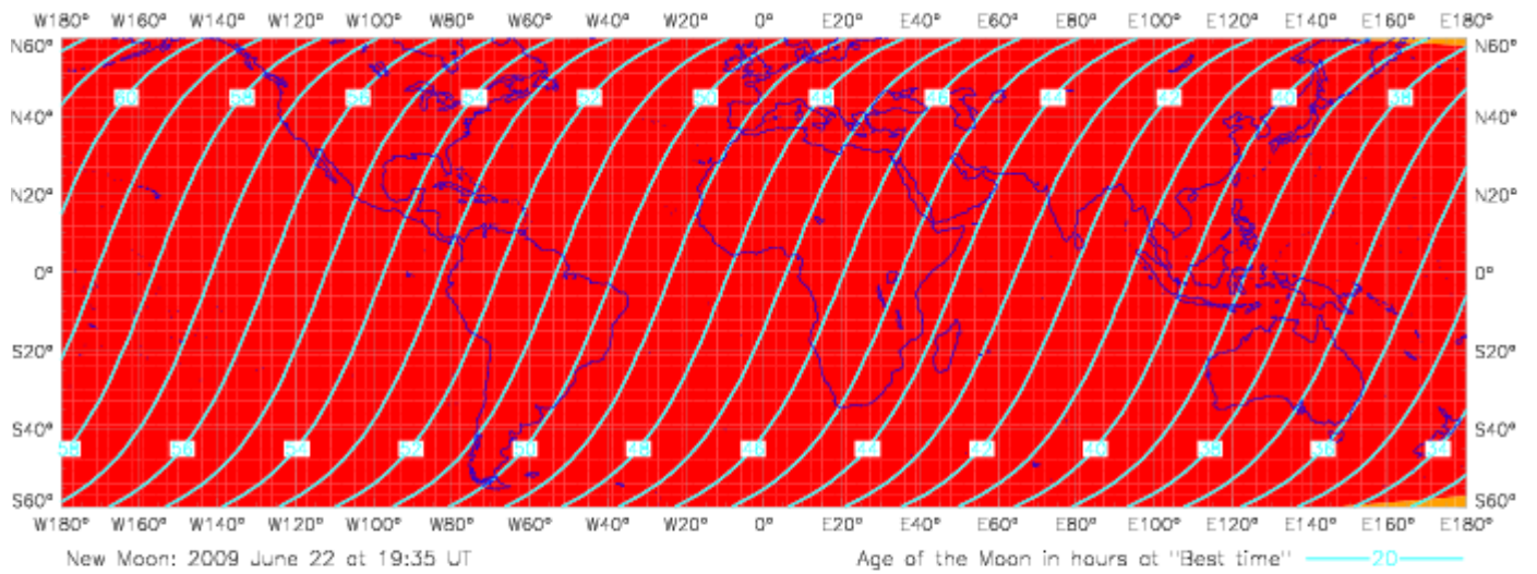
Visibility of the New Crescent Moon for 2009 June 24
